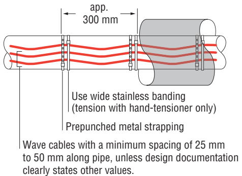
Figure 15: Fastening several runs of cable
