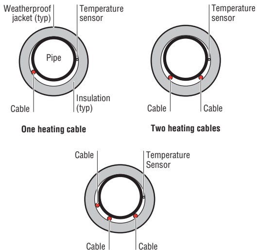
Figure 6 : Cable orientation on pipe
