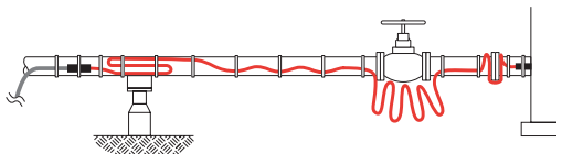
Figure 12: Installing cable on valves and pipe supports
