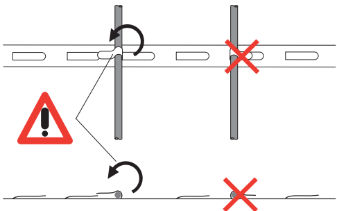
Figure 8: Fixing device: pre-punched metal strap
