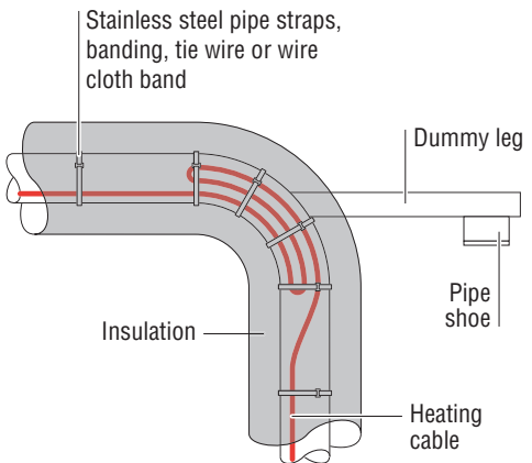
Figure 21: Dummy supports
