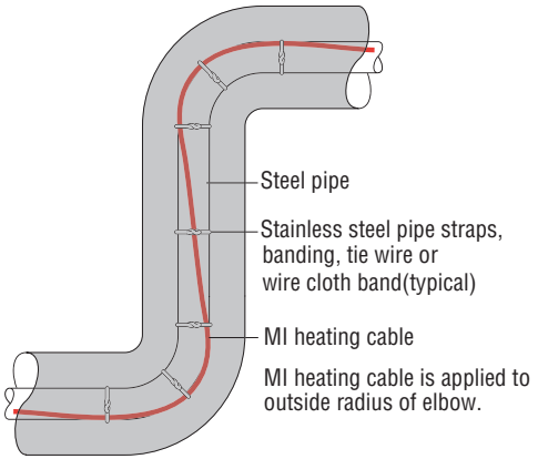
Figure 17: Installation at 90° elbow
