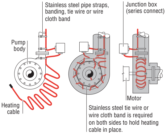
Figure 22: Pumps
