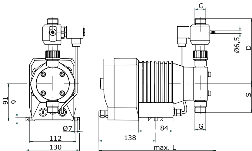
(Abmessungen CS 204.1-1,2e ...-14e, PVC, PP, PVDF) (Dimensions CS 204.1-1,2e ...-14e, PVC, PP, PVDF)
